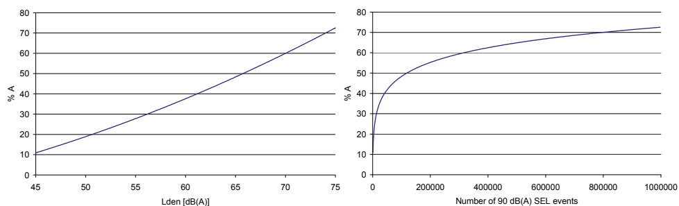
Fig. 8. The Miedema dose-response relation plotted against L_{den} in dB(A) as well as against a number of annual 90 dB(A) SEL events
