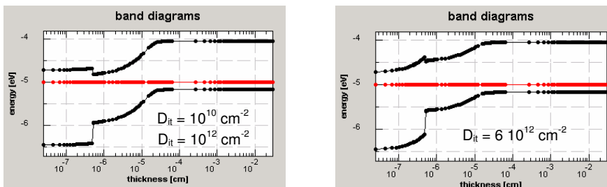
Fig. 6. Screenshots of equilibrium band diagrams (red: Fermi energy, black: valence and conduction band energy) for three different a-Si:H/c-Si interface state densities D_{it} .
