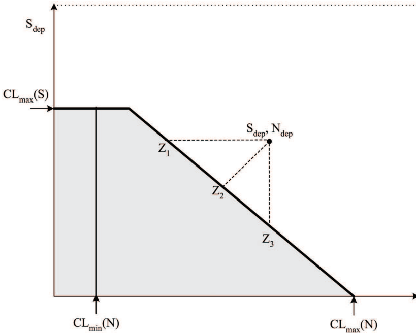
Fig. 1. The critical load function of acidity
