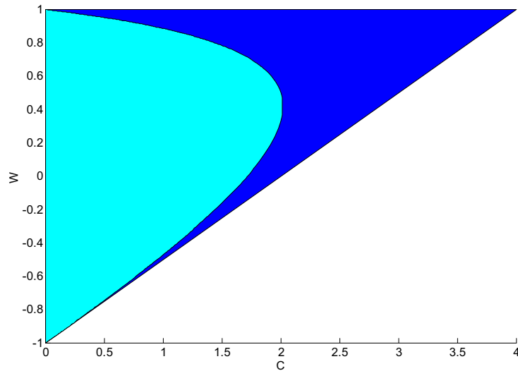
Figure 4 Relationship between \omega and c when c_1=c_2=c to simultaneously guarantee the convergence of iterative processes \{EX_t\} and \{DX_t\}
