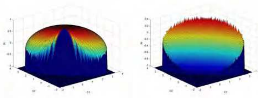
Figure 3 Relationship between lower(left) and higher(right) range of \omega and c_1, c_2 to guarantee the convergence of iterative process \{DX_t\}
