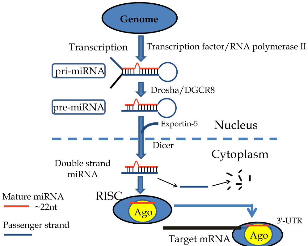
Fig. 1. Biogenesis of miRNA
