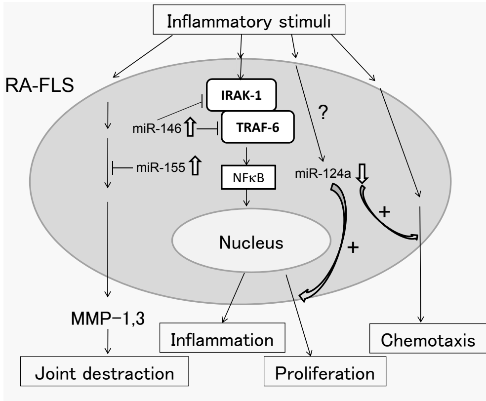
Fig. 2. The role of miRNAs in RASF
