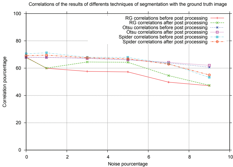
Fig. 12. Correlation of different segmentation techniques.
